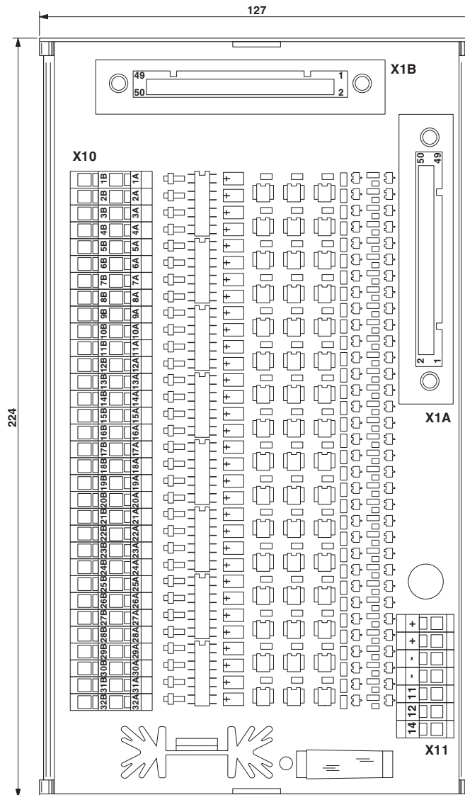
Dimensional drawing
