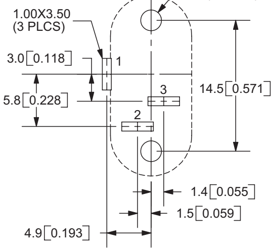
PCB LAYOUT FRONT VIEW
