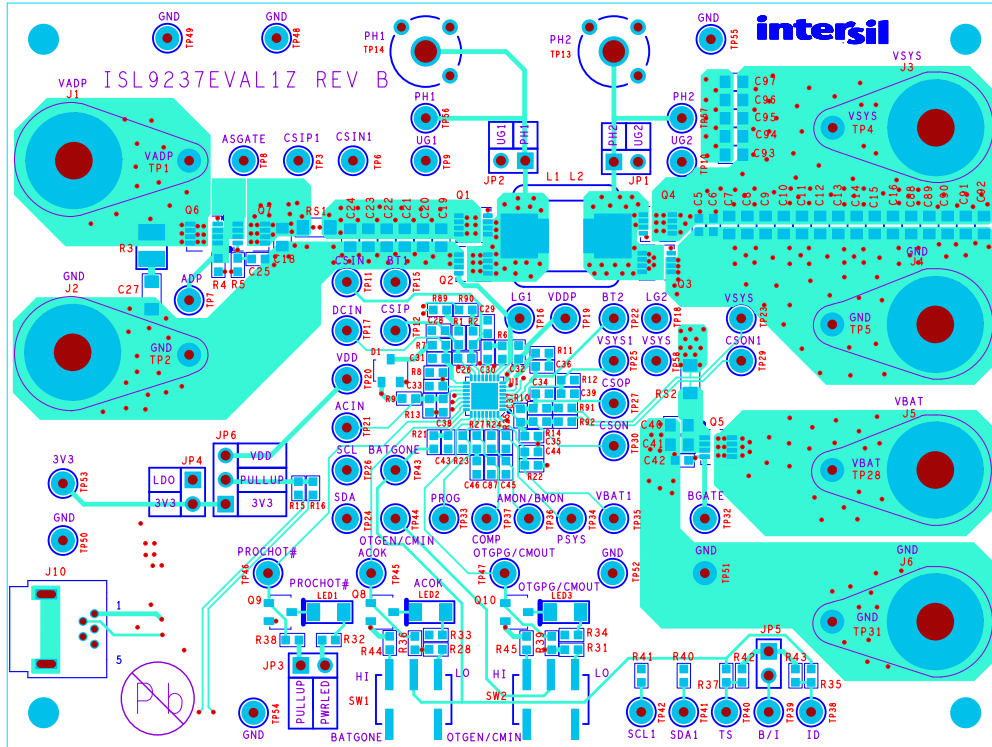
FIGURE 9. TOP LAYER
