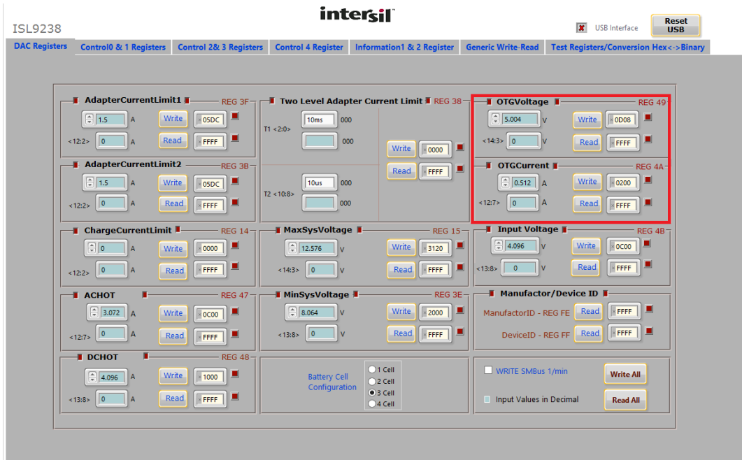
FIGURE 4. OTG VOLTAGE AND CURRENT SETTING IN GUI
