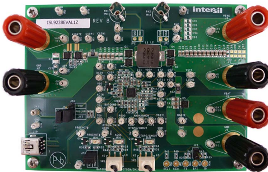
FIGURE 7. TOP OF BOARD
