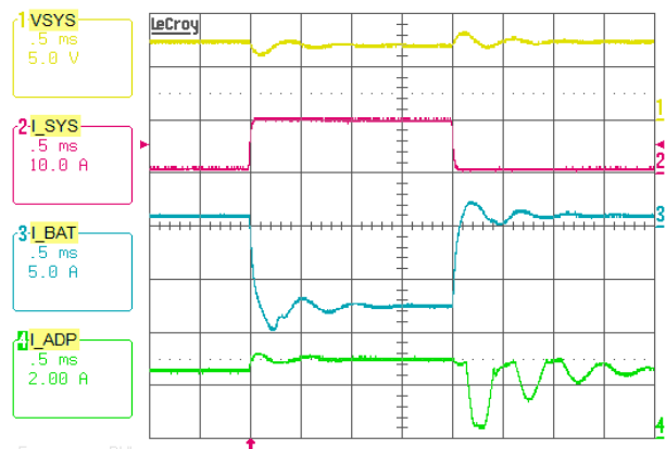
FIGURE 14. BOOST MODE, CHARGING CURRENT LOOP TO ADAPTER CURRENT LOOP TRANSITION. V_{ADP} = 5V , MAXSYSTEMVOLTAGE = 8.496V , V_{BAT} = 7V , SYSTEM LOAD 0.5A TO 10A STEP, ADAPTERCURRENTLIMIT = 3A, CHARGECURRENT = 1A
