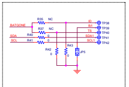
FIGURE 6. ISL9238EVAL1Z BOARD SCHEMATIC
