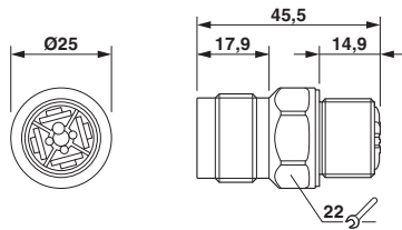
Dimensional drawing
