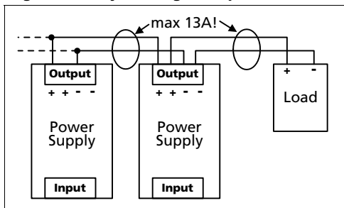
Fig. 23-5 Daisy chaining of outputs
