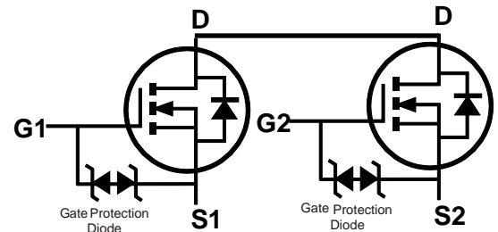
Equivalent Circuit
