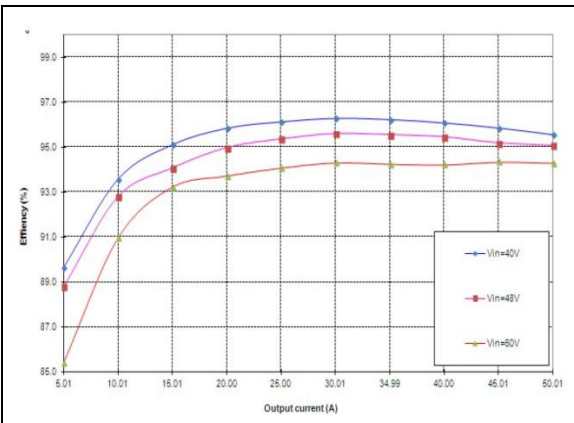
Figure 9: ADQ600-48S12-6L Efficiency Curves @ 25 °C
