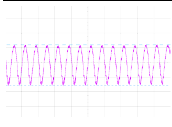
Figure 2: ADQ600-48S12-6L Ripple and Noise Measurement Ch : Vo (5µs/div, 30mV/div)
