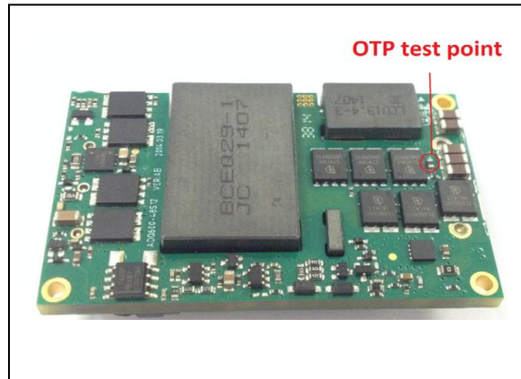
Figure 10: ADQ600-48S12-6L Over Temperature Protection Test Point
