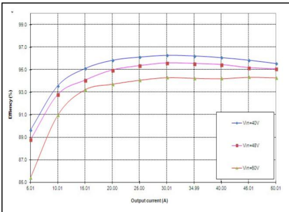
Figure 19: ADQ600-48S12B-6L Efficiency Curves @ 25 degC Loading: Io = 10% increment to 50A
