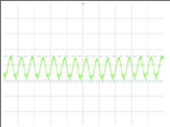
Figure 1: ADQ600-48S12-6L Input Reflected Ripple Current Waveform Ch : Iin (5µs/div, 40mA/div)
