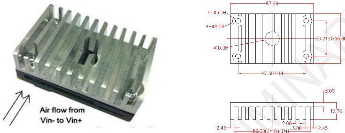
Figure 25 Typical test condition with heat sink
