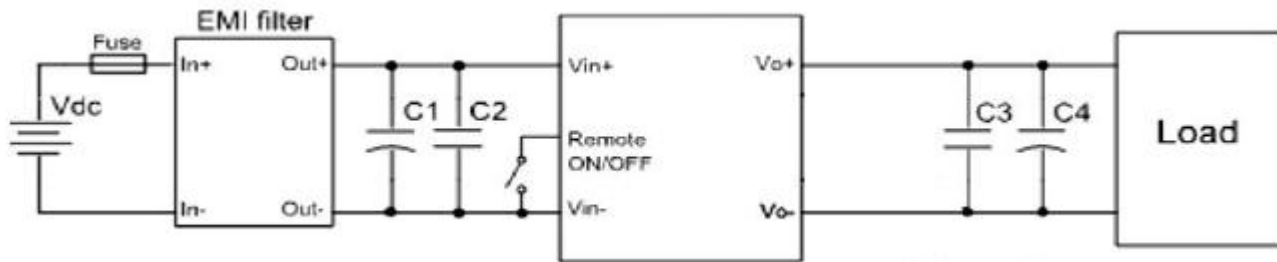
Figure 27 Typical application
