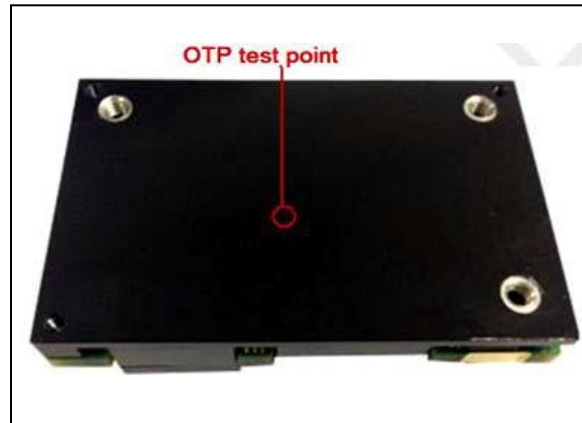
Figure 20: ADQ600-48S12B-6L Over Temperature Protection Test Point
