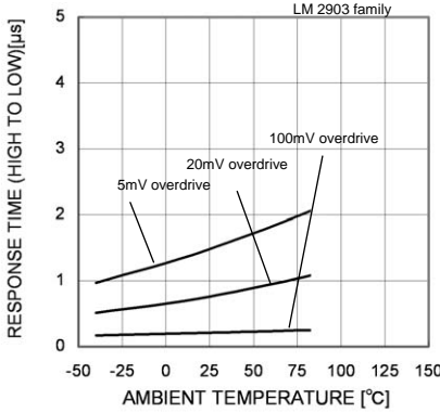
Fig. 63 Response Time (High to Low) – Ambient Temperature
