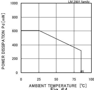
Fig. 64 Derating Curve
