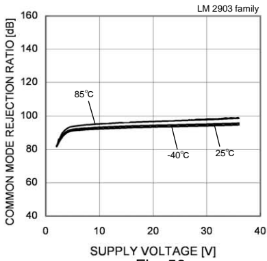
Fig. 56 Common Mode Rejection Ratio – Supply Voltage
