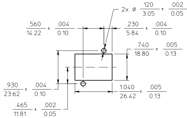
VIEW B RECOMMENDED MOUNTING HOLES SCALE: 1:1
