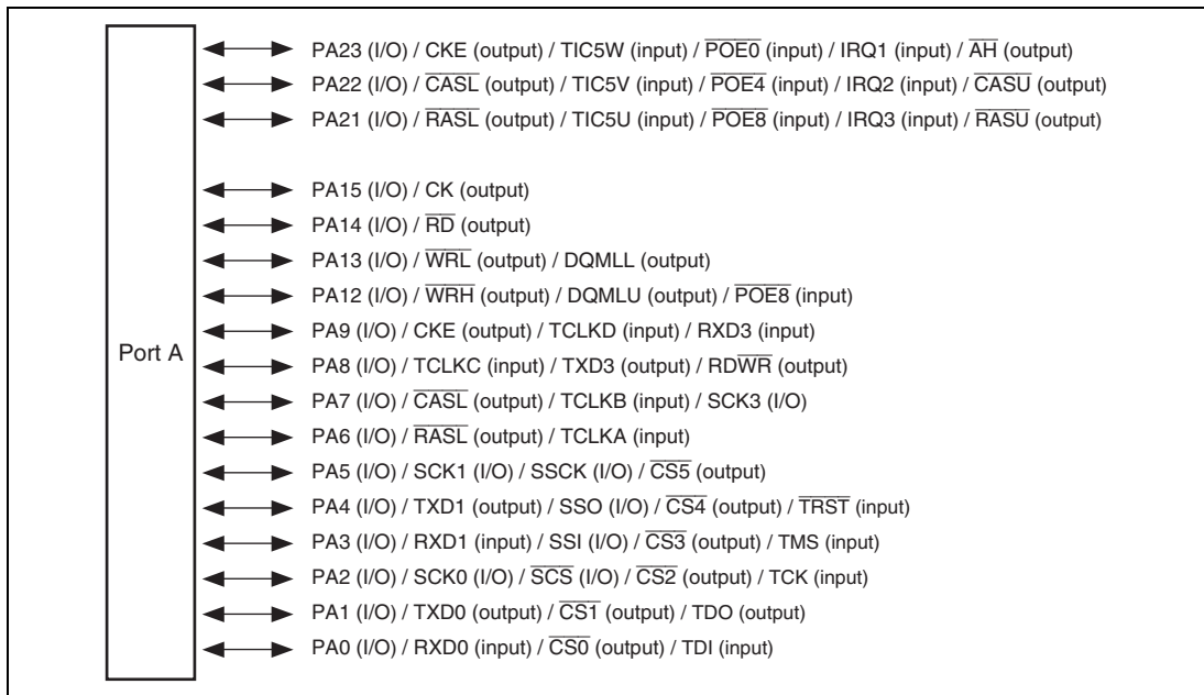
Figure 24.2 Port A (SH7285)
