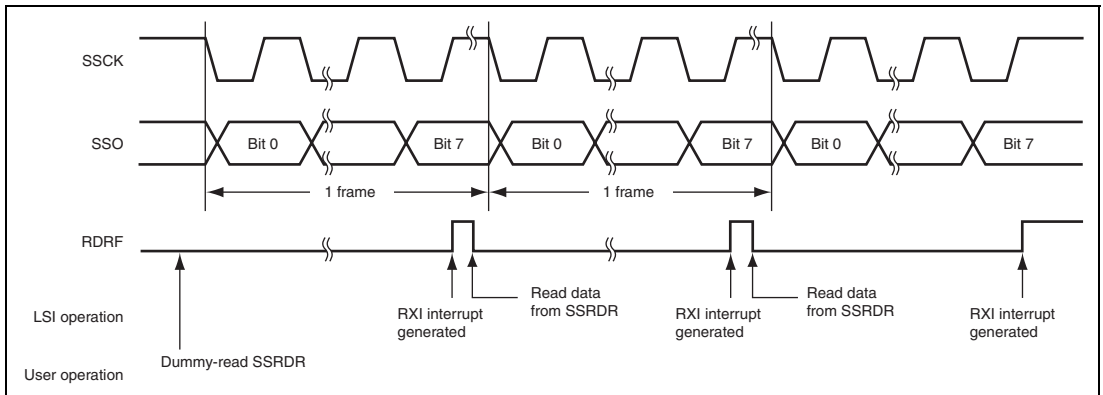
Figure 18.15 Example of Reception Operation (Clock Synchronous Communication Mode)
