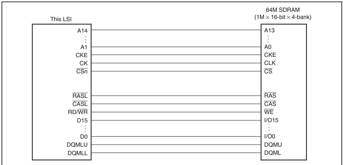
Figure 9.16 Example of 16-Bit Data Width SDRAM Connection
