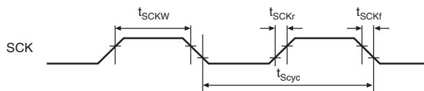
Figure 31.47 SCK Input Clock Timing
