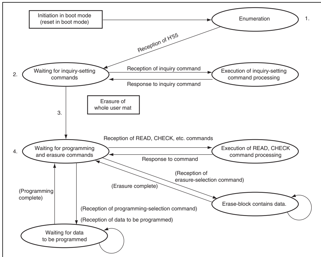
Figure 26.10 USB Boot Mode
