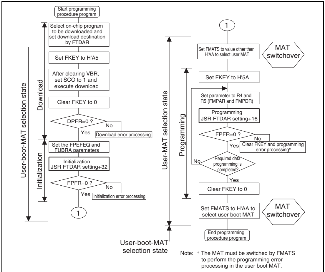
Figure 26.16 Procedure for Programming User MAT in User Boot Mode
