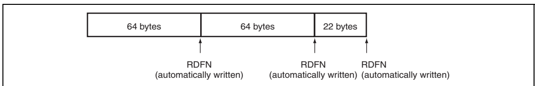
Figure 25.22 EP1 RDFN Operation
