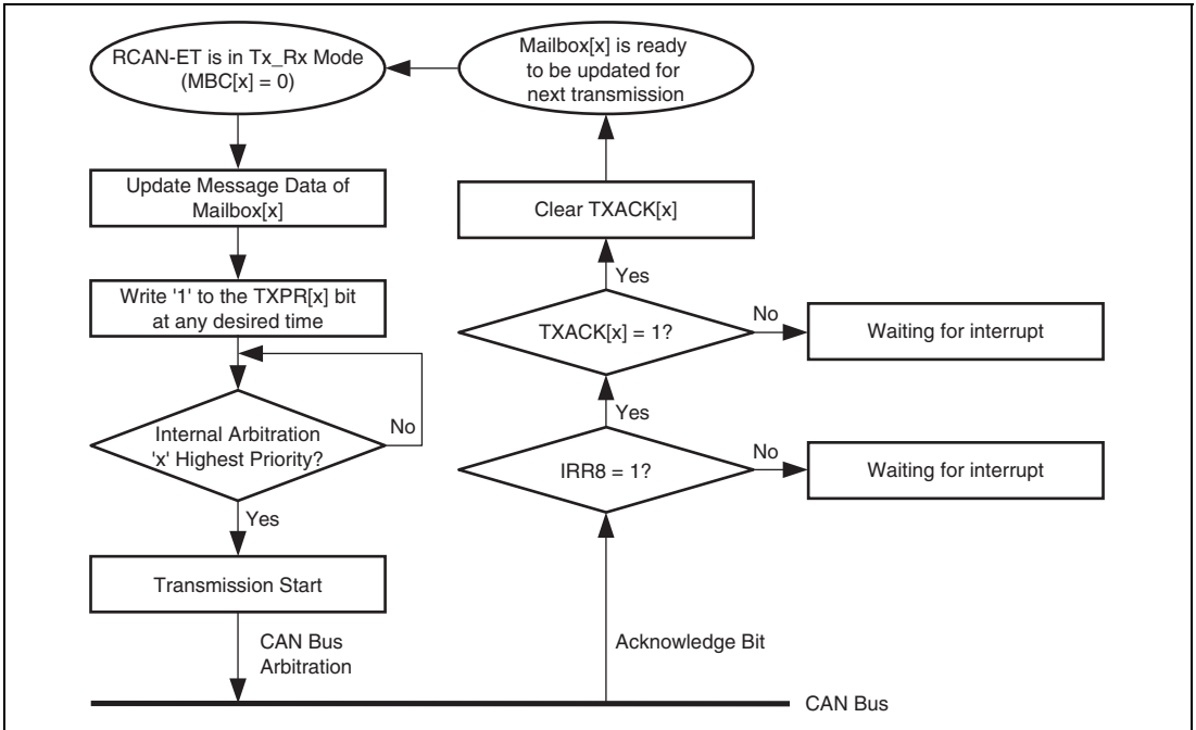
Figure 22.10 Transmission Request
