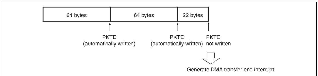
Figure 25.19 EP2 PKTE Operation
