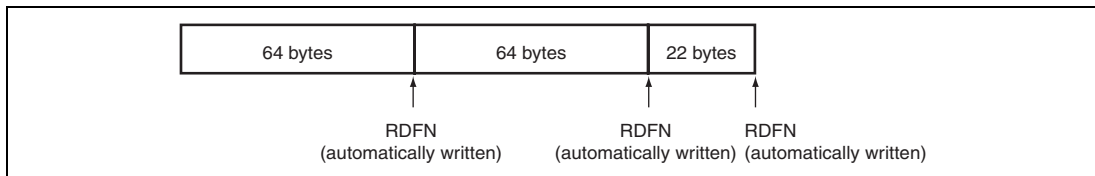
Figure 25.16 EP1 RDFN Operation
