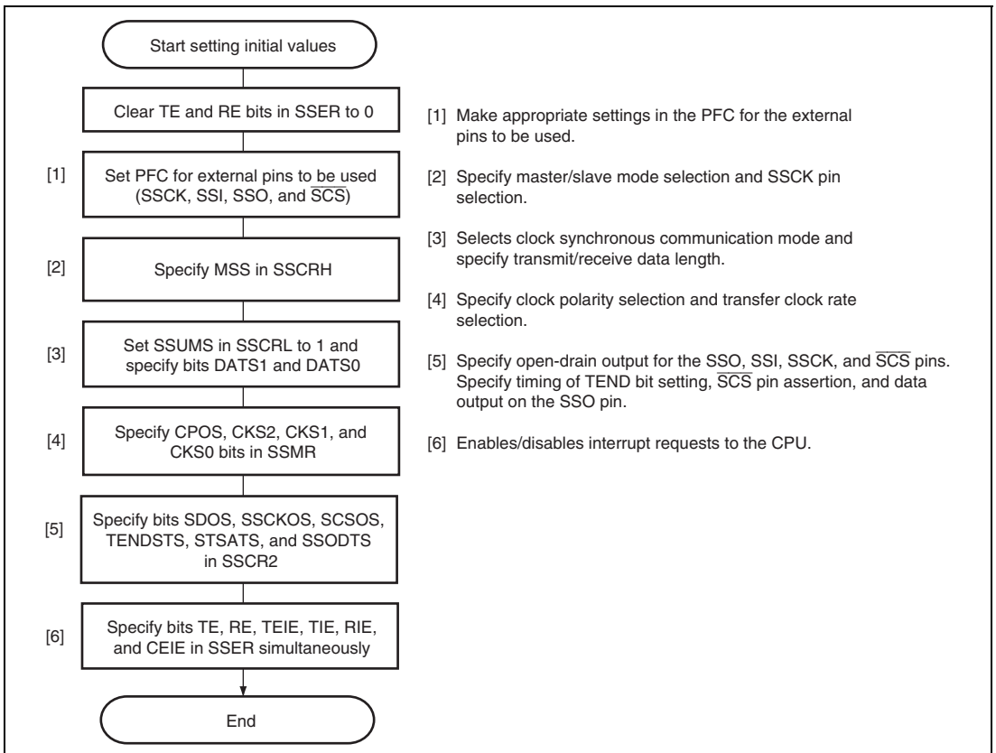
Figure 18.12 Example of Initial Settings in Clock Synchronous Communication Mode
